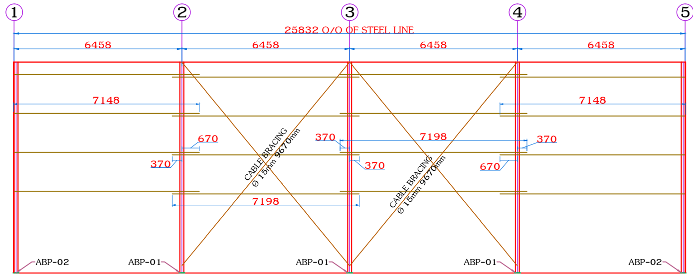
SIDE WALL FRAMING @ GRID-D
