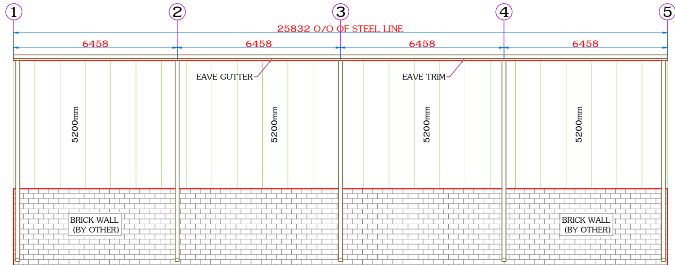
SIDE WALL SHEETING @ GRID-D
